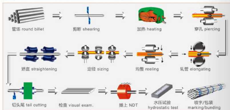
热轧钢管生产工艺流程图 Hot-rolling Pipe Process Diagram
