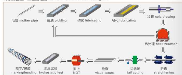
冷拔钢管生产工艺流程图 Cold-drawn Pipe Process Diagram
