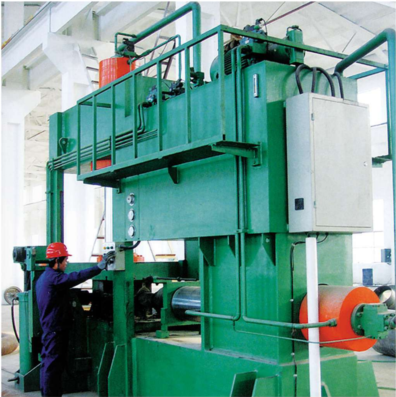
不锈钢弯头推制设备 Stainless steel elbow pushing equipment
